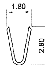
B-B SECTION
